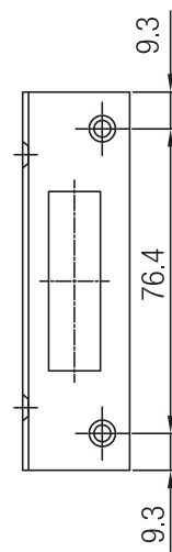
Striking plate Thickness: 1,5 mm
